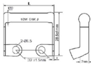
“L” type terminal-TMOL
