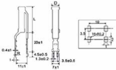
Vertical type-TMOV
